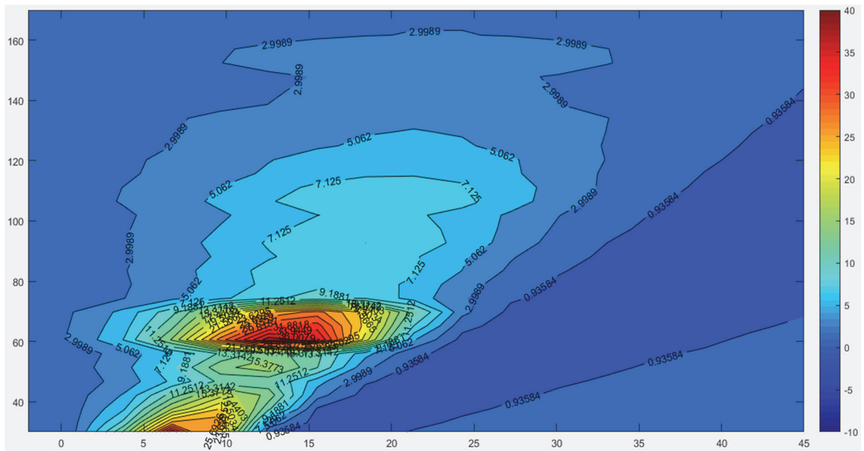
Fig. 4. Permeability distribution of overlying strata (y=-3m~45m, h=30m~170m)
