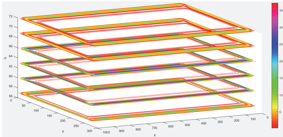
Fig. 5. Isocline of Permeability in 57m, 60m, 63m and 72m over coal seam
