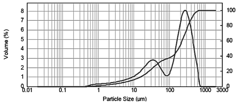
Fig.3. Quartz sand particle size distribution, peaks at 300 and 35μm
