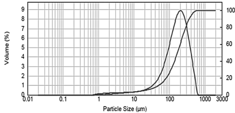
Fig. 1. Particle size distribution coarse CRT panel glass, is show a peak at 200μm
